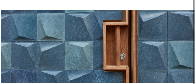
3D facade panel wastewater cellulose, reed and calcite
